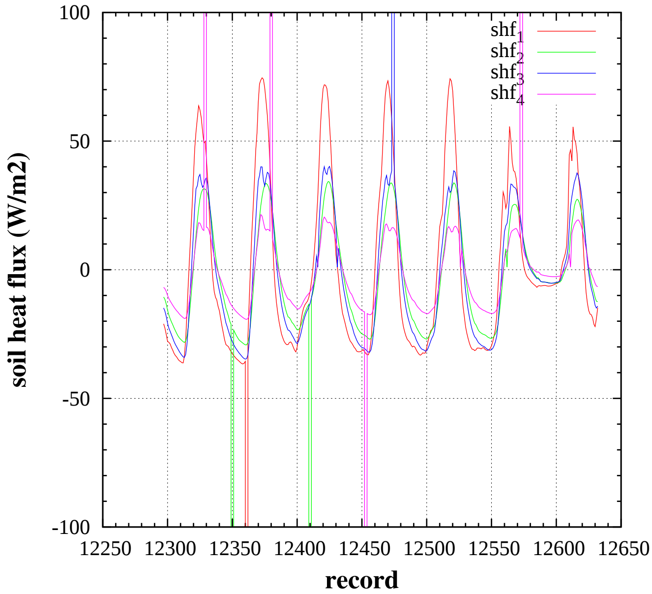
Soil heat flux Raimat 23 Gen a 1 Mar 2009
