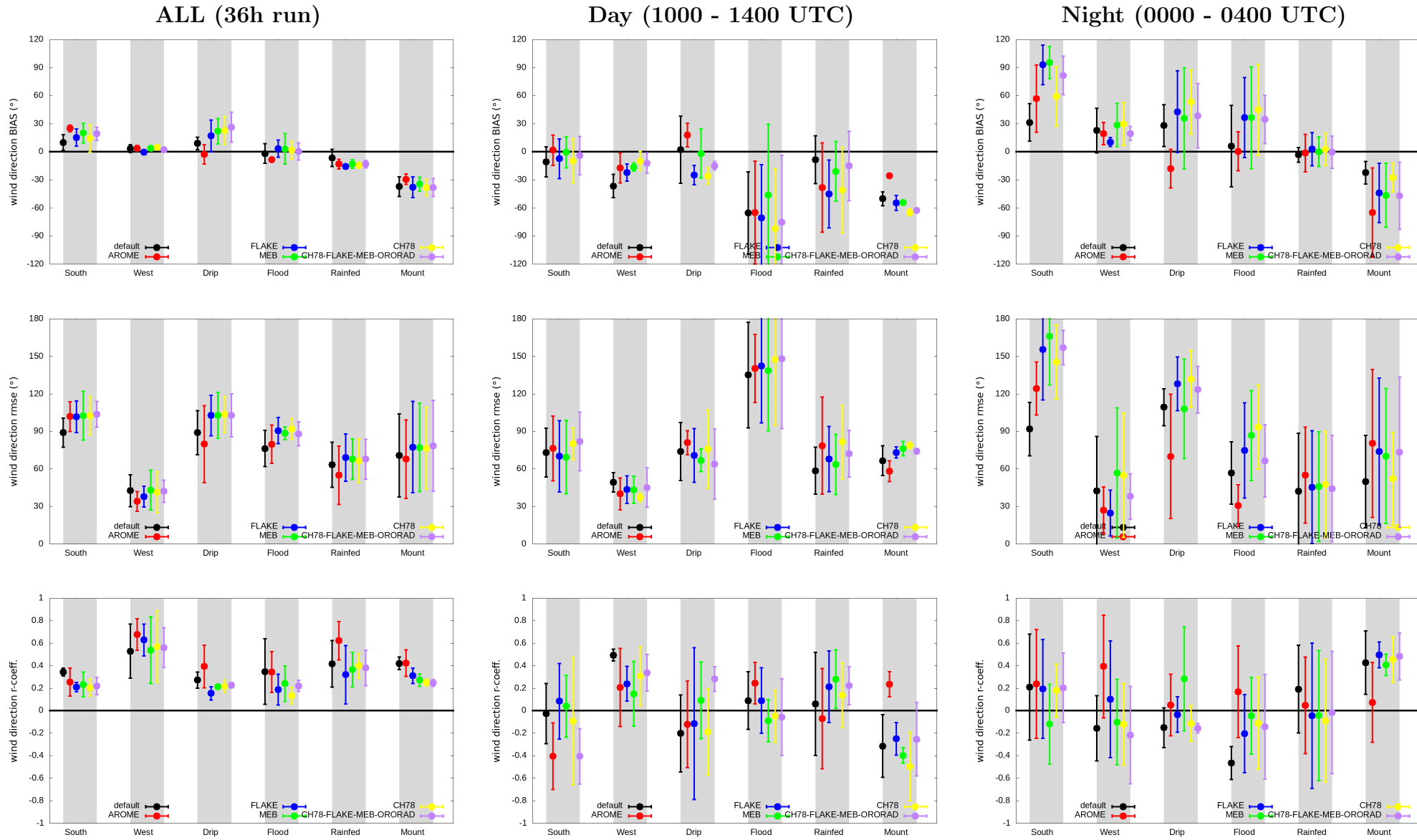
Figure 2: Wind direction statistics averaged over the 6 selected regions.
