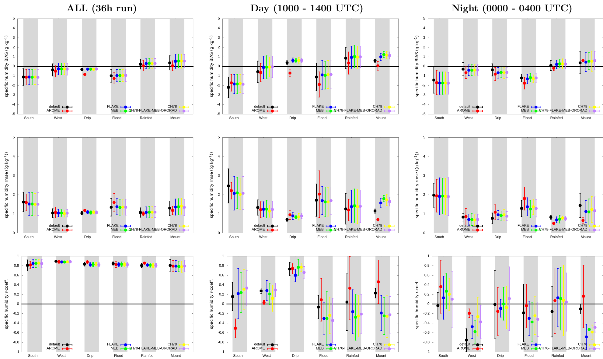
Figure 4: Specific humidity statistics averaged over the 6 selected regions.
