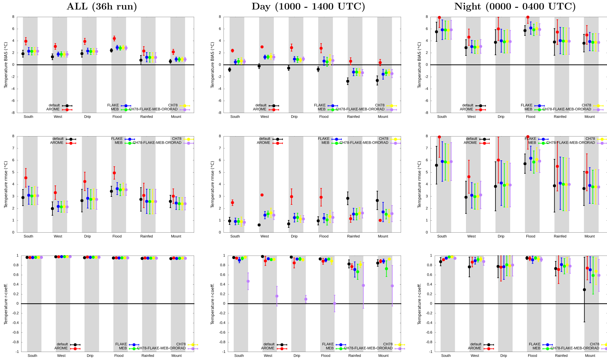
Figure 3: Temperature statistics averaged over the 6 selected regions.
