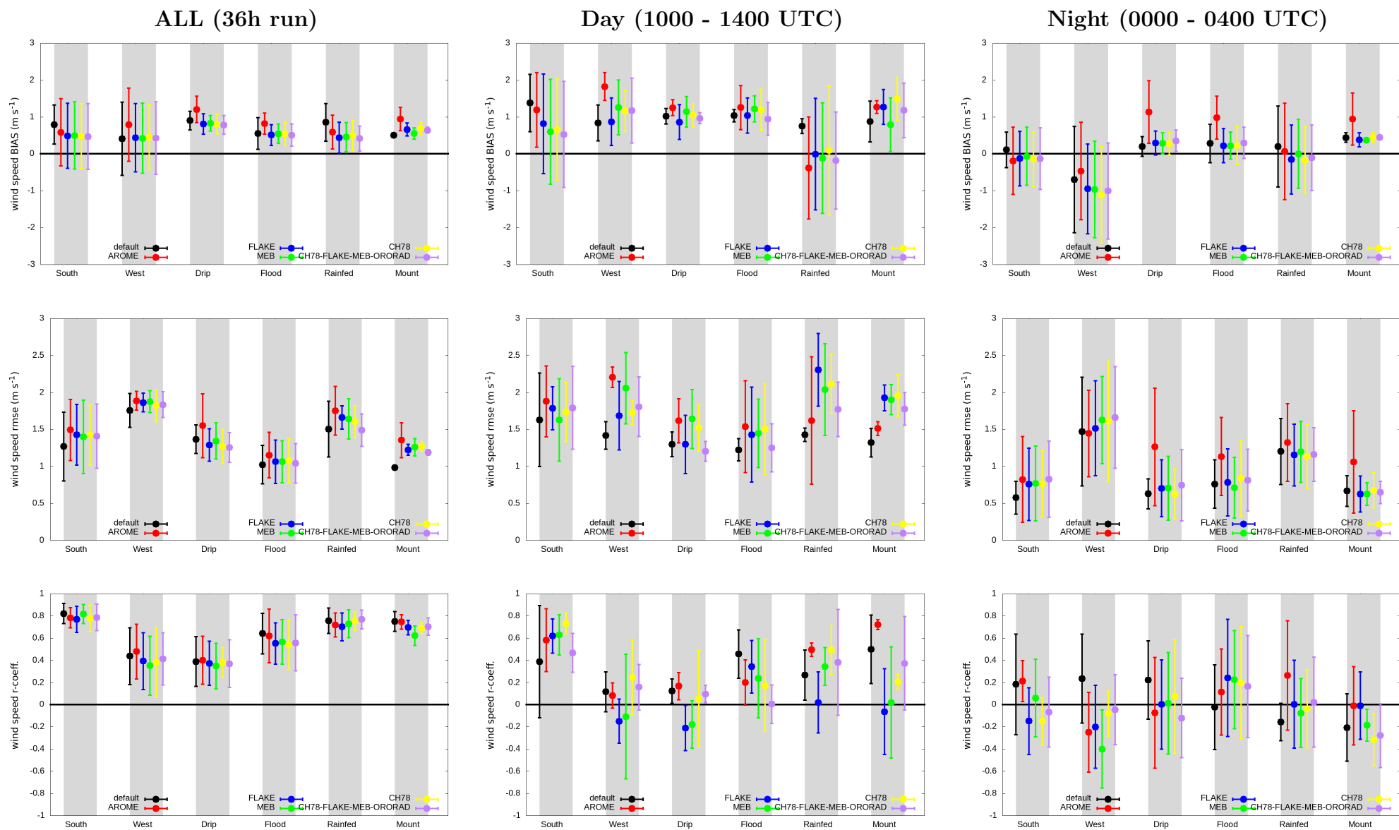
Figure 1: Wind speed statistics averaged over the 6 selected regions.
