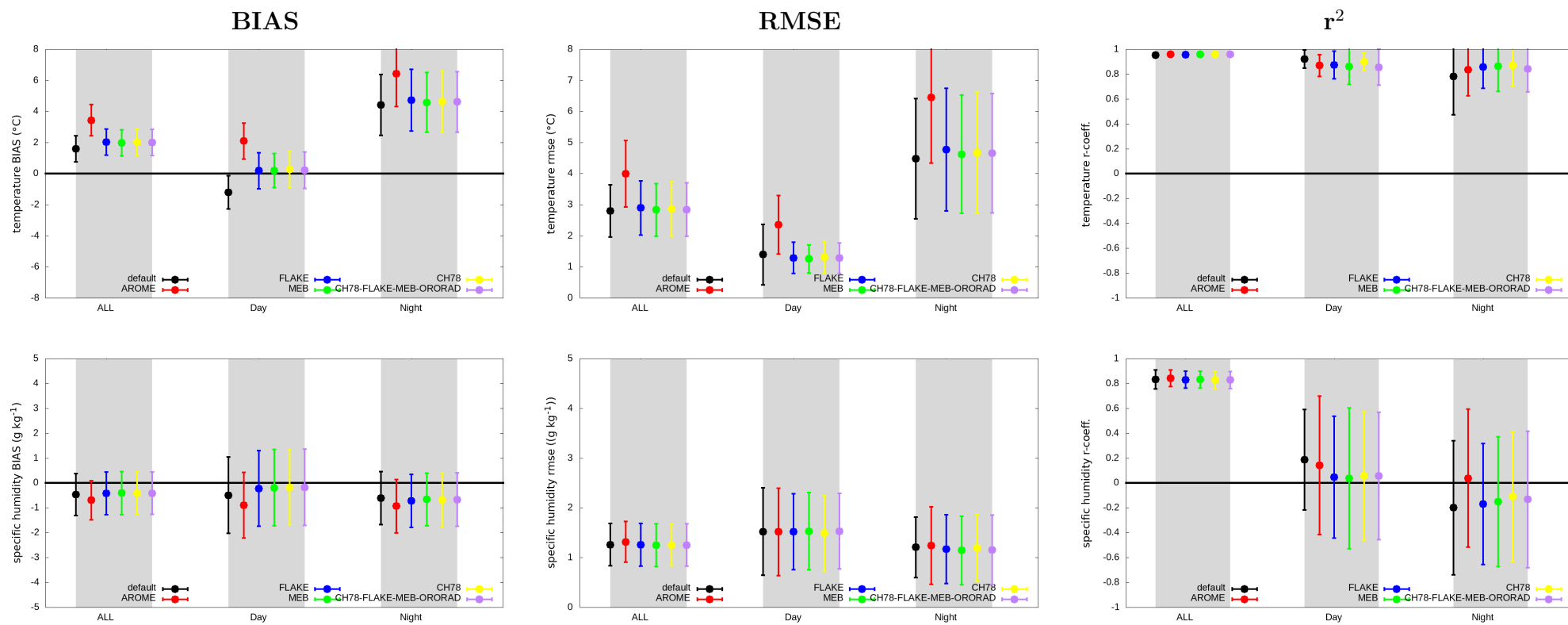
Figure 2: Temperature and specific humidity statistics averaged over all the AWS over the studied region.
