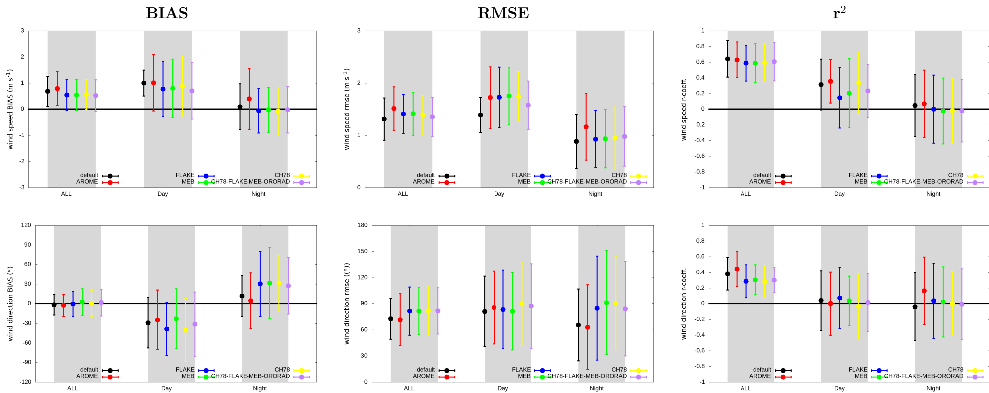
Figure 1: Wind speed statistics averaged over all the AWS over the studied region.
