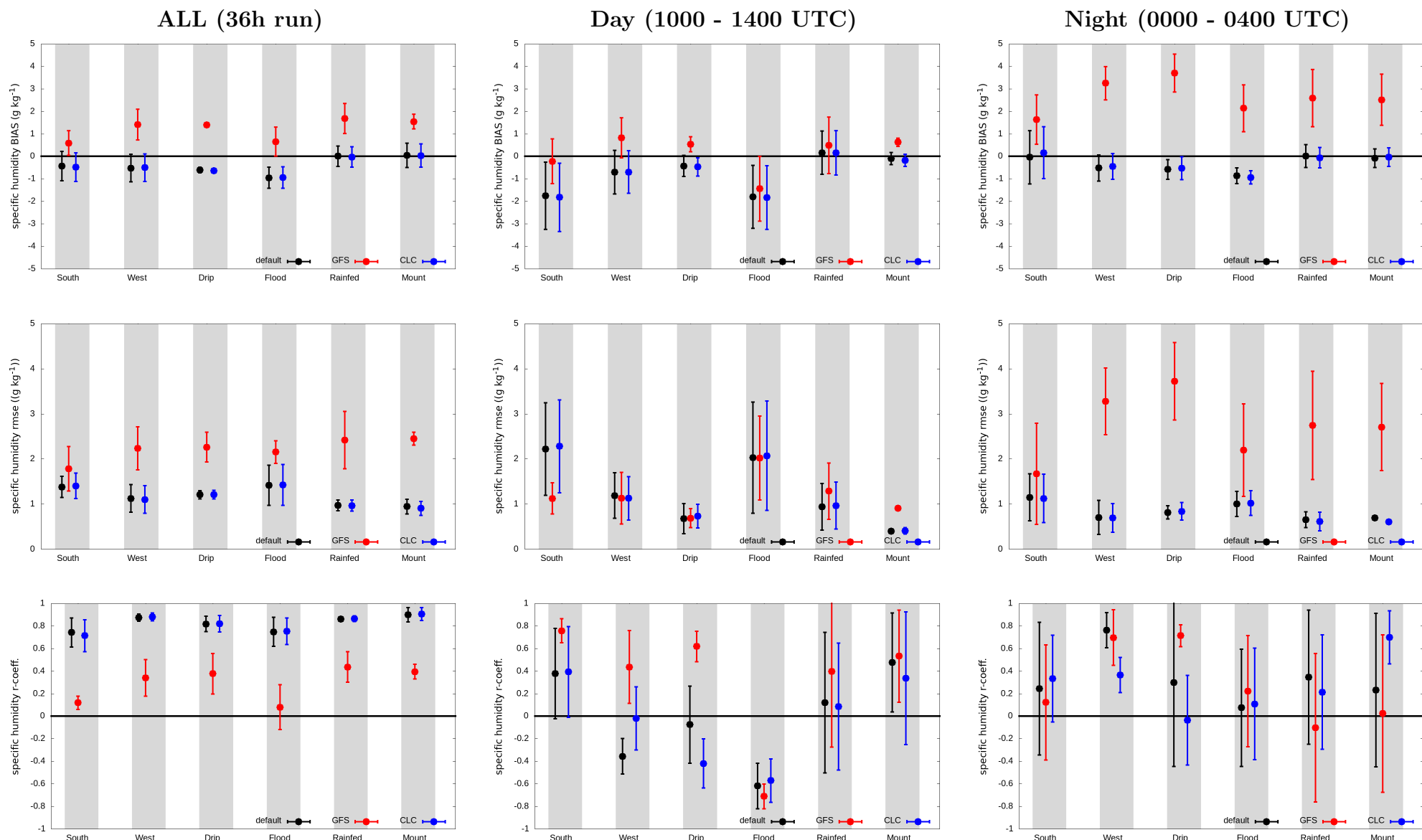
Figure 4: Specific humidity statistics averaged over the 6 selected regions.
